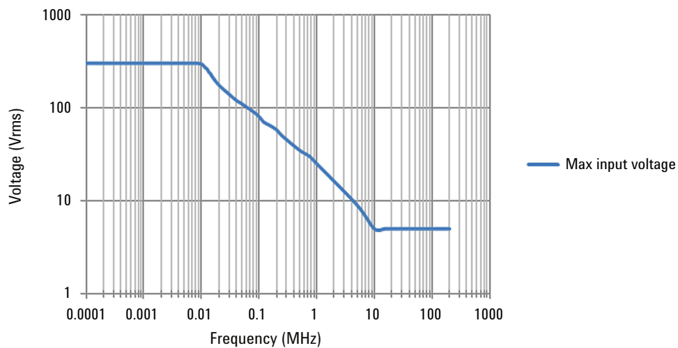
Figure 6. Maximum input voltage
